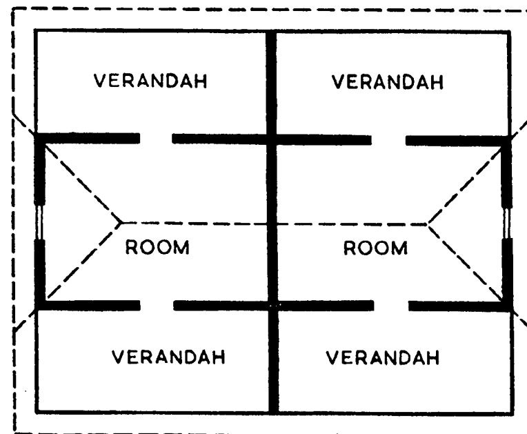
GROUND PLAN OF A COLONY HOUSE
