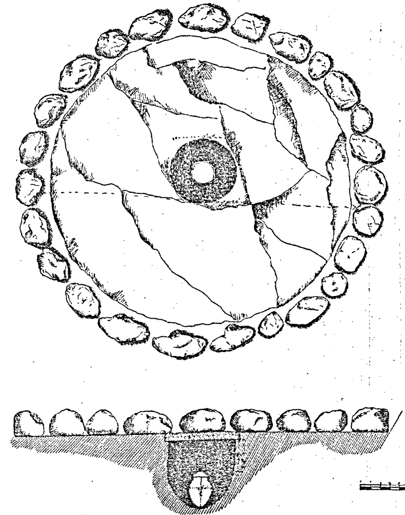
GROUND PLAN & SECTION OF AN URN BURIAL, PUDUKKOTTAI
